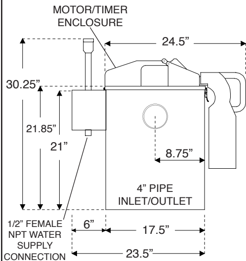
END VIEW
